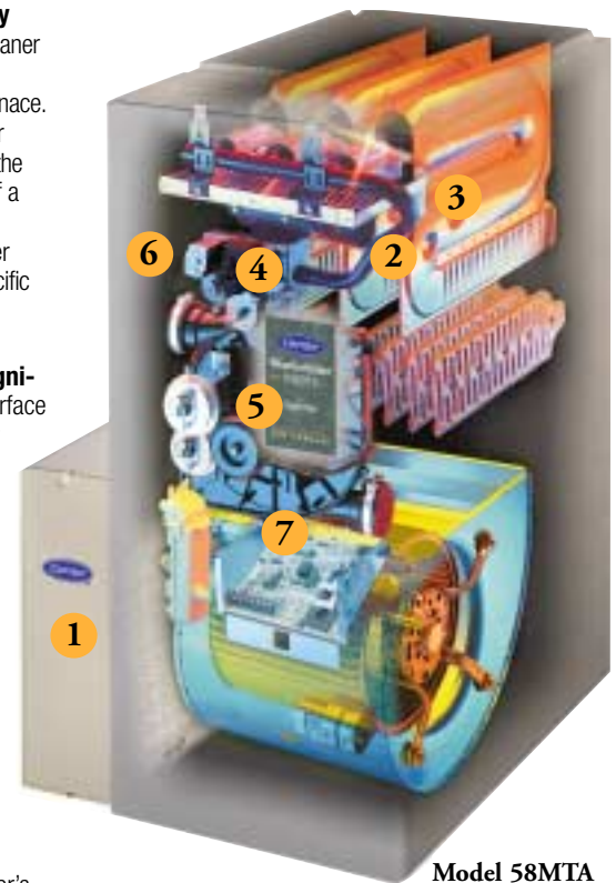
Model 58MTA
